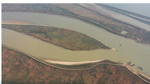
Sediment of distributary channel in the central Jiangxi branch of the Ganjiang Delta
